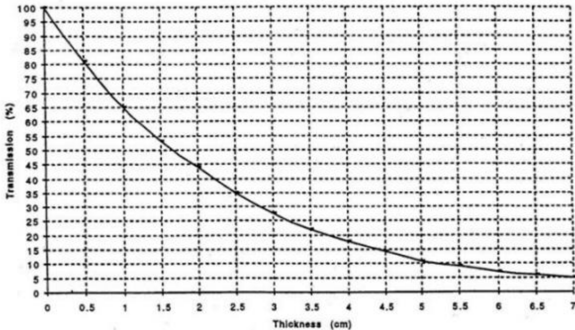
Cerrobend Transmission for 18MV photons
